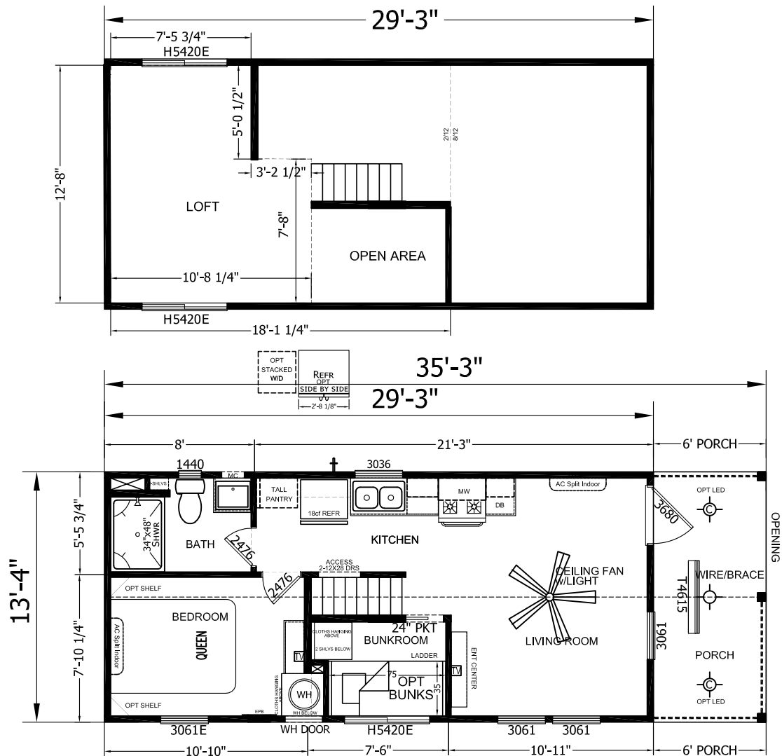
ATHENS PARK 4110L 2 BEDROOM 1 BATH 29'-3" x 13'-4" 398 SQ. FT. TOTAL
